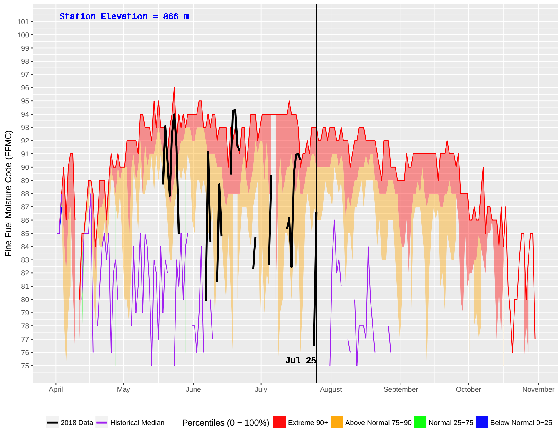
CATFISH (199) : Historical (1986–2016) and Current (2018) Noon Fine Fuel Moisture Code (FFMC)
